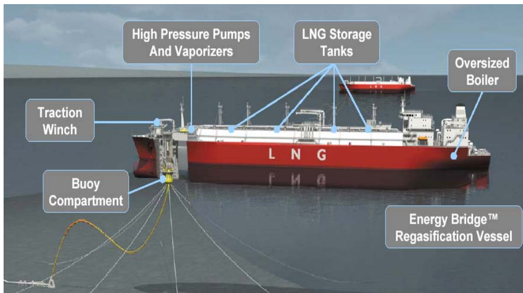
Figure 31 – LNG Tanker Serving Gulf Gateway Terminal 86
