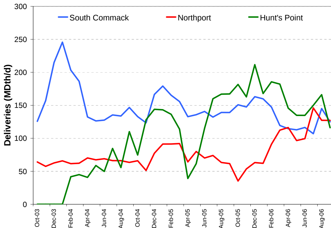
Figure 9 – Average Monthly Iroquois Deliveries to Long Island and New York City
